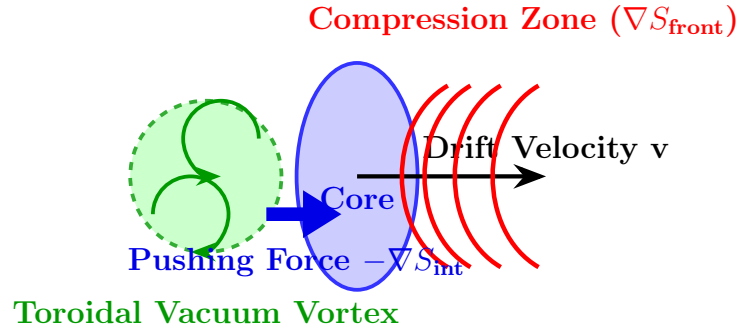
Figure 2: The autowave mechanism of electronic motion: The trailing toroidal gyroscopic vortex of vacuum bubbles collapses behind the defect, generating the internal scalar pressure gradient \nabla S that sustains inertial flight.
