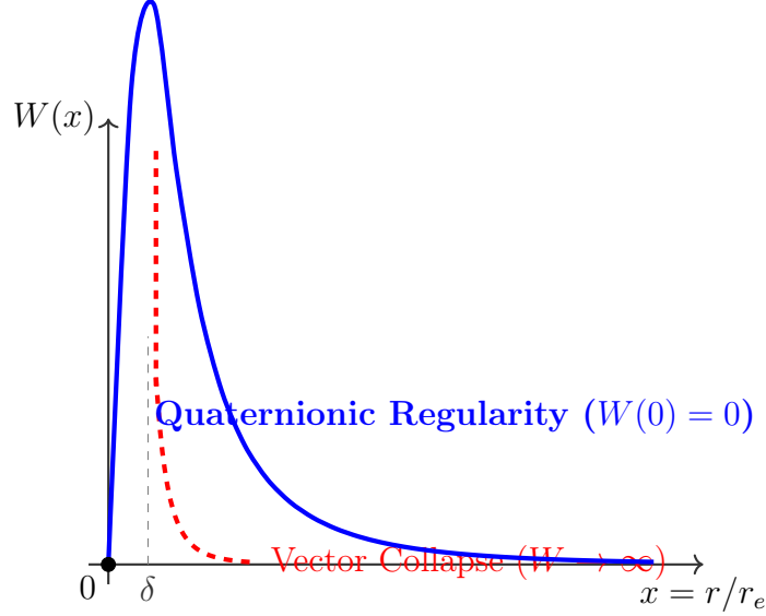
Figure 1: Radial distribution of local energy density W(x) : Classical vector singularity explosion versus smooth quaternionic stabilization inside the vortex core.
